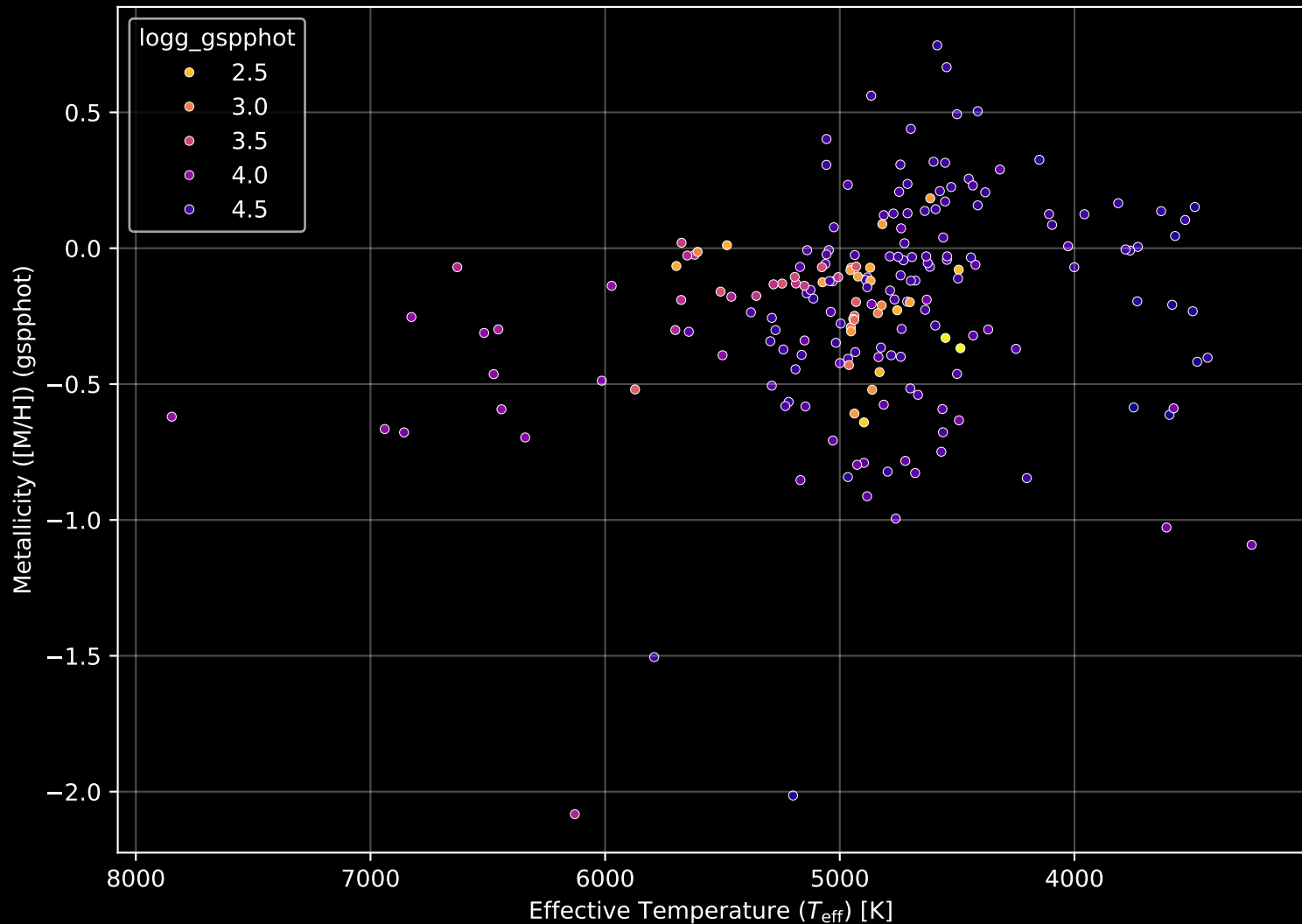
APOGEE DR17 Field: [K2_C8_117-58_btx] Stellar Population Parameters (n= 199)
