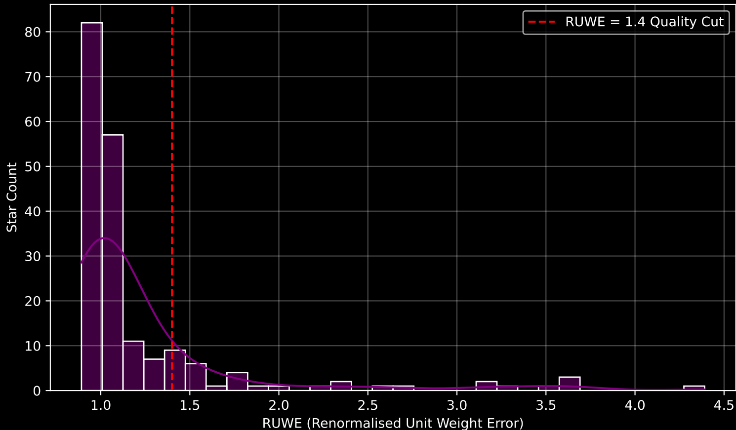
GAPOGEE DR17 Field [K2_C8_117-58_btx] RUWE Distribution (n= 192)
