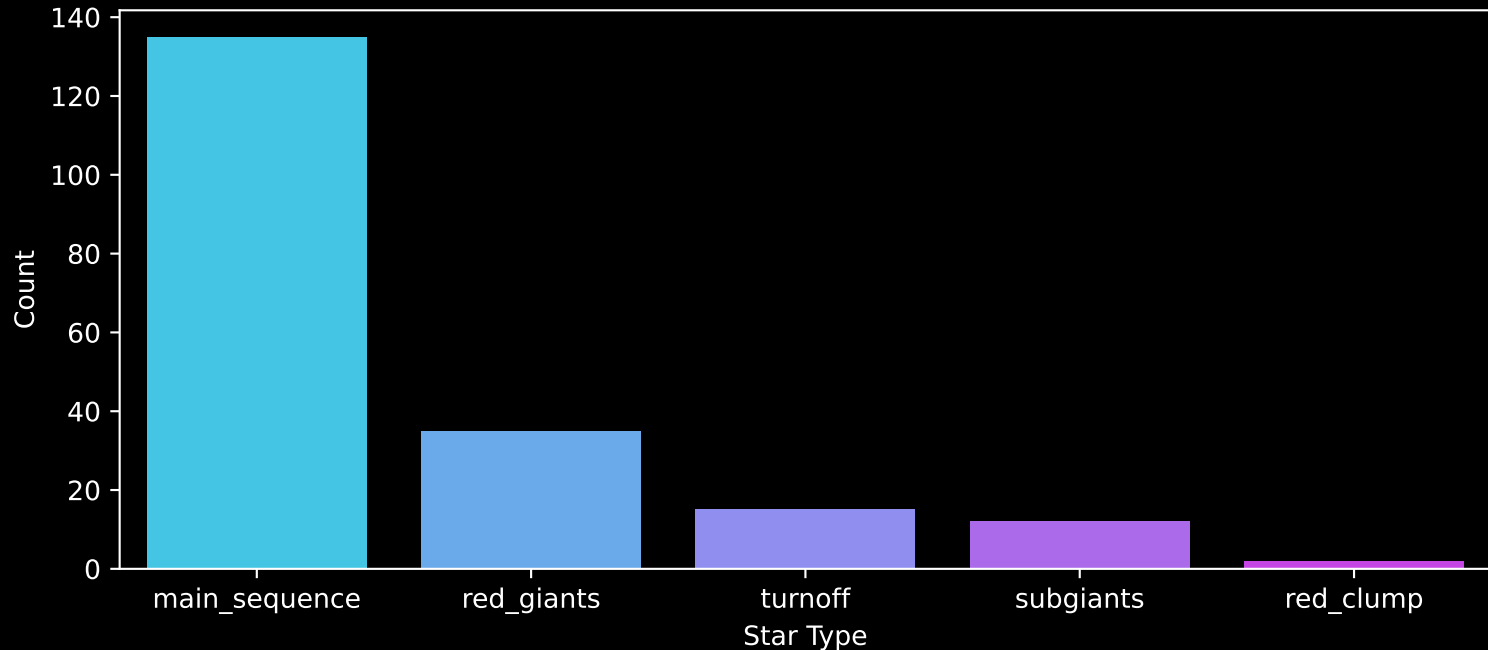
APOGEE DR17 Field: [K2_C8_117-58_btx] Count plot of Star Type
