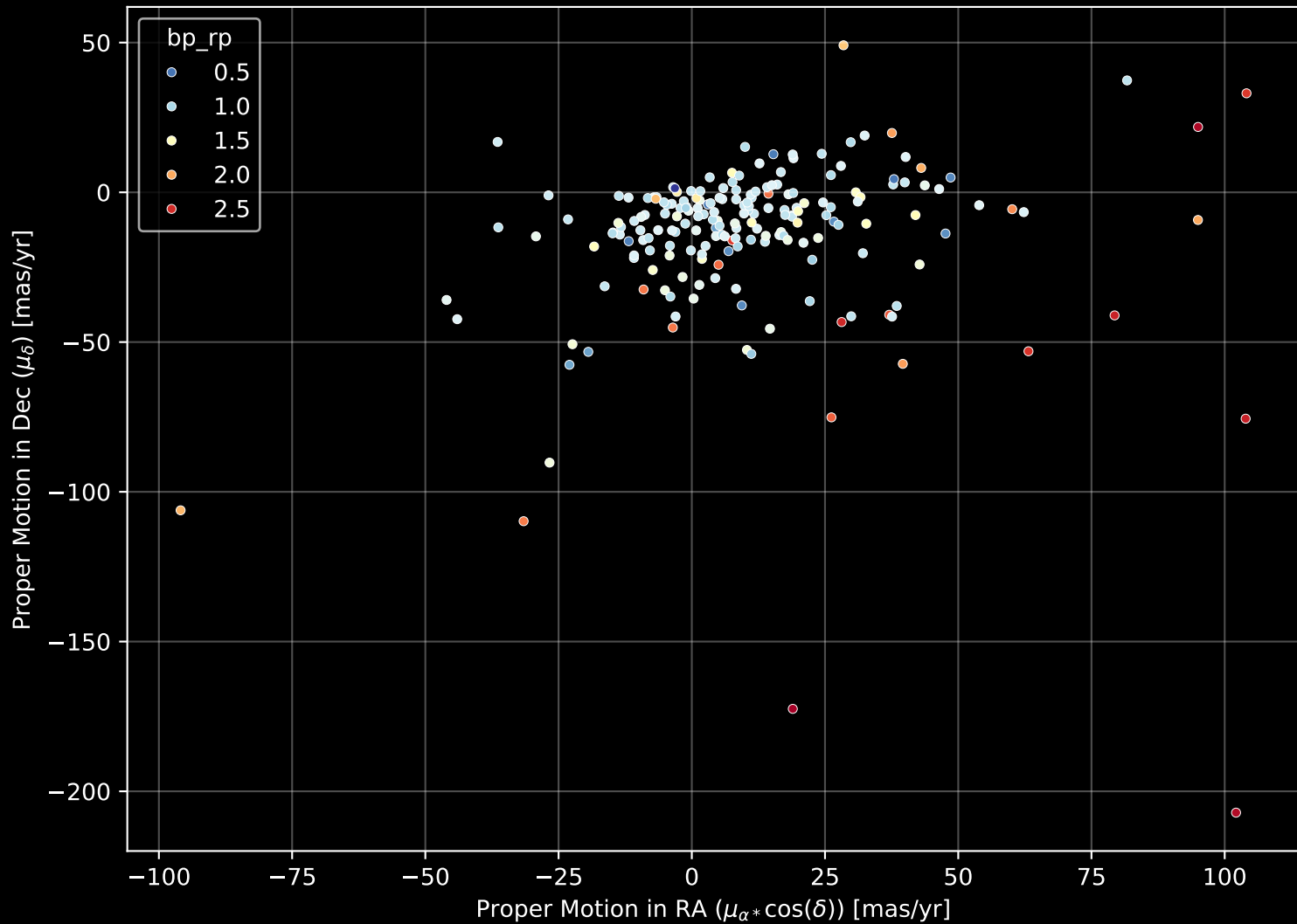
APOGEE DR17 Field: [K2_C8_117-58_btx] Proper Motion Diagram (n= 199)
