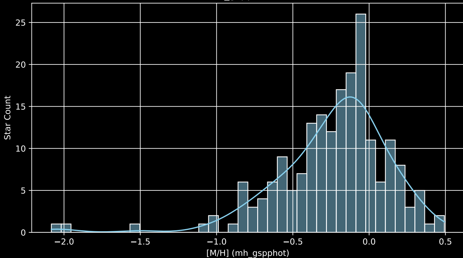
APOGEE DR17 Field: [K2_C8_117-58_btx [M/H] (mh_gspphot) (n= 195)
