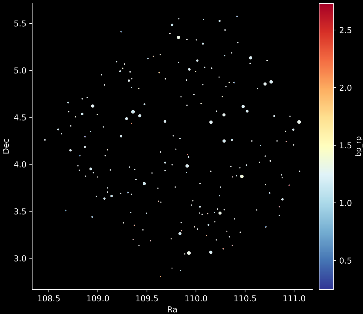
APOGEE DR17 Field: [K2_C8_117-58_btx] Stars: 199
