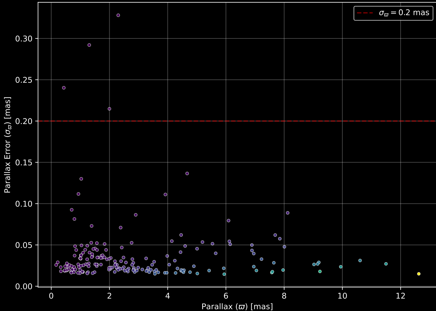
APOGEE DR17 Field: [K2_C8_117-58_btx] Parallax Quality (n= 199)
